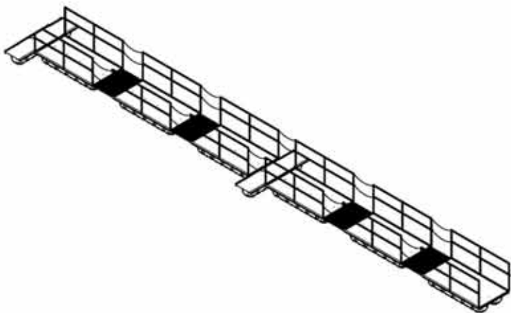
Design layout of long span walkway with stabiliser and grating insert
