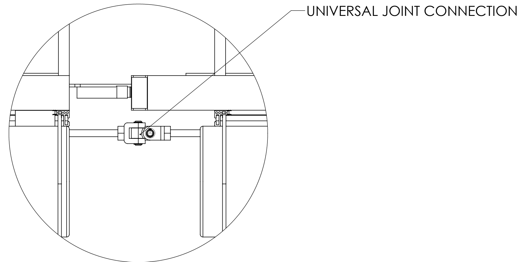
DETAIL A SCALE 1 : 8
